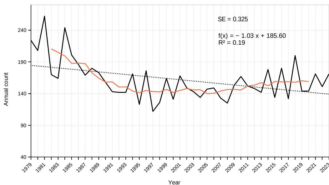
Fig. 2. The annual number of E macroform (black line). The trend line (dotted black line), regression equation, R^2 , standard error of the slope coefficient (SE) and 7-year moving average (red line) have been added
