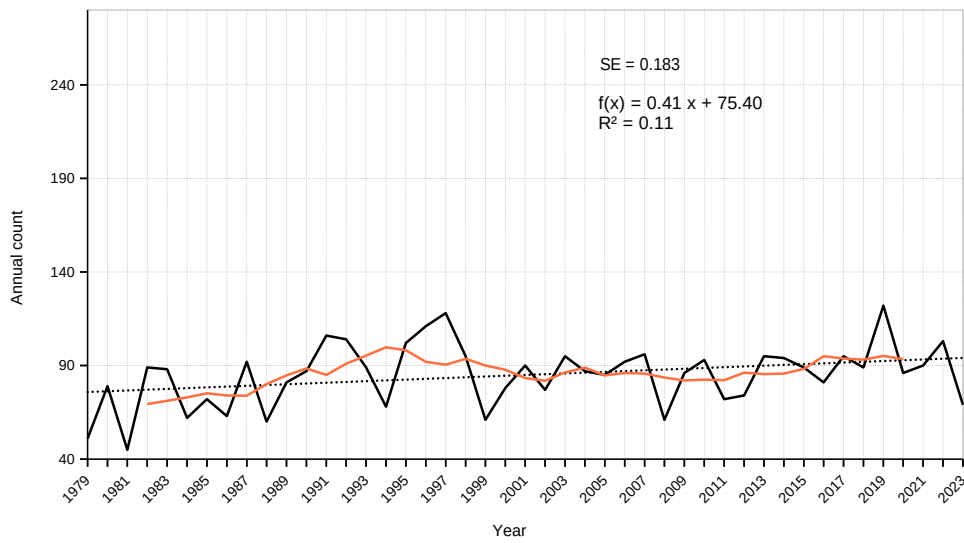
Fig. 3. The annual number of C macroform (black line). The trend line (dotted black line), regression equation, R^2 , standard error of the slope coefficient (SE) and 7-year moving average (red line) have been added
