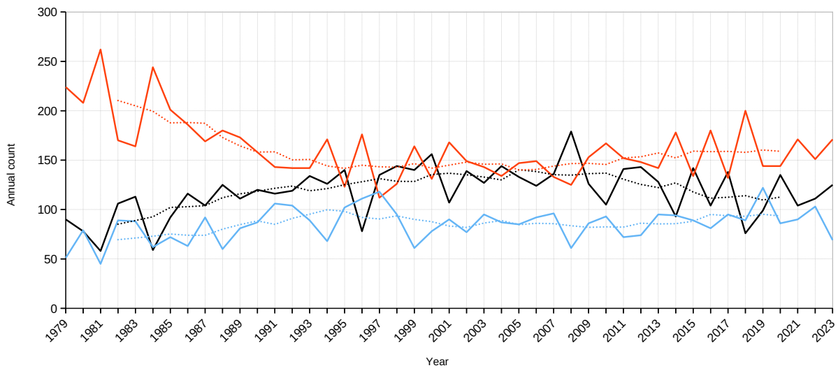
Fig. 5. The annual number of W (black line), E (red line), and C (blue line) macroforms in the period 1979–2023. The dotted lines mark 7-year moving average
