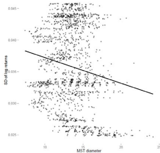
Figure 4. Scatterplot of MST diameter vs st. dev. of log returns
