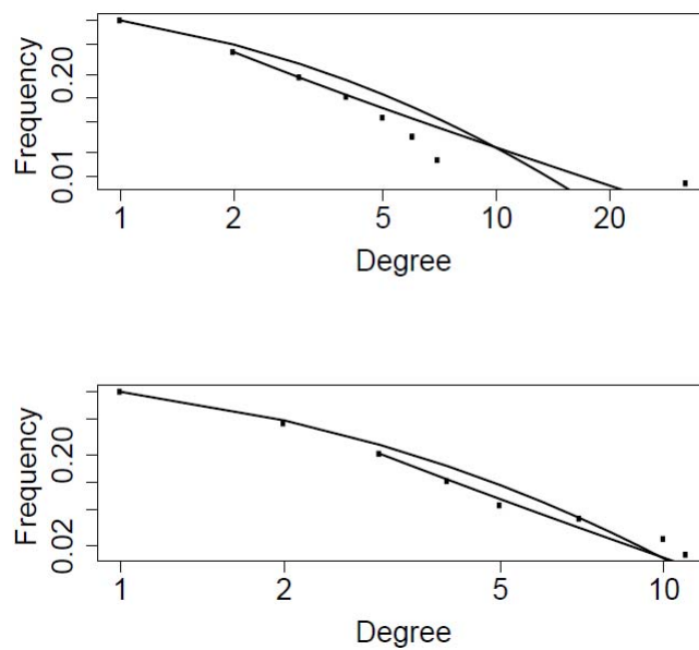
Figure 7. Degree distributions for two specific MST with power law and log-normal distributions fitted
