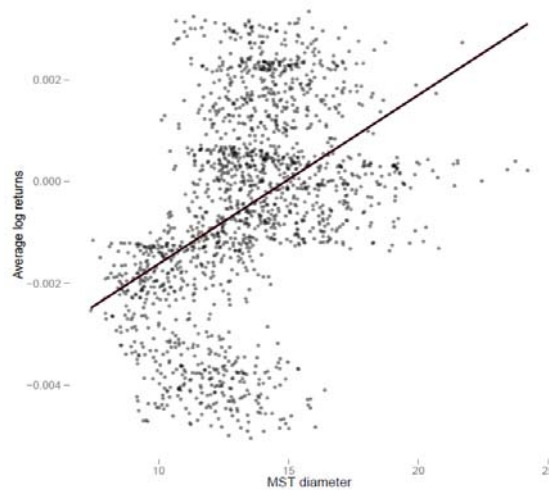
Figure 3. Scatterplot of average log returns vs MST diameter
