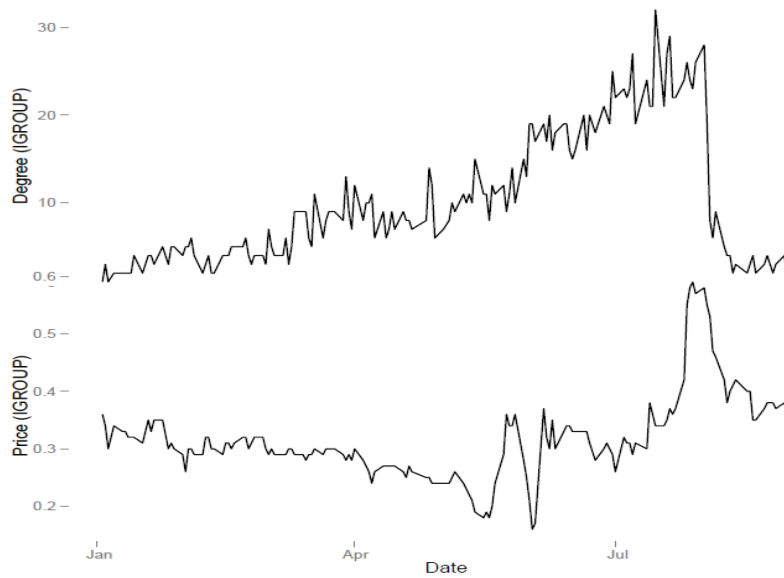
Figure 6. Changes in price and degree of IGROUP in the MST
