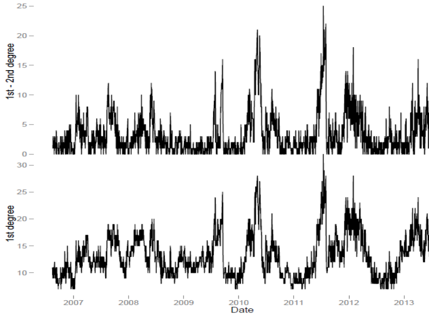
Figure 5. Changes in highest degree and difference between highest and second highest degree within the MST over time
