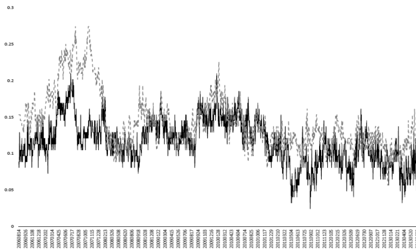
Figure 1. Percentage of intrasector links in all links within constructed MST over time Source: author's calculations
