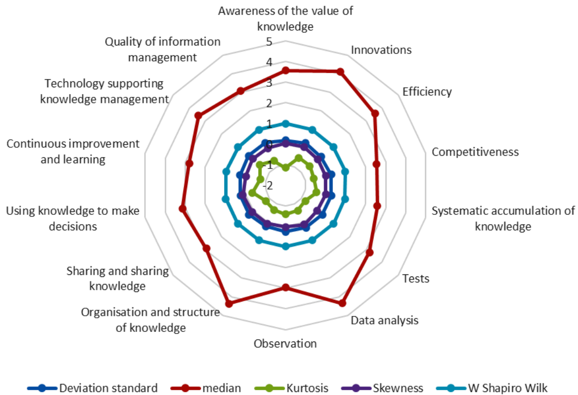
Figure 2. Descriptive statistics
